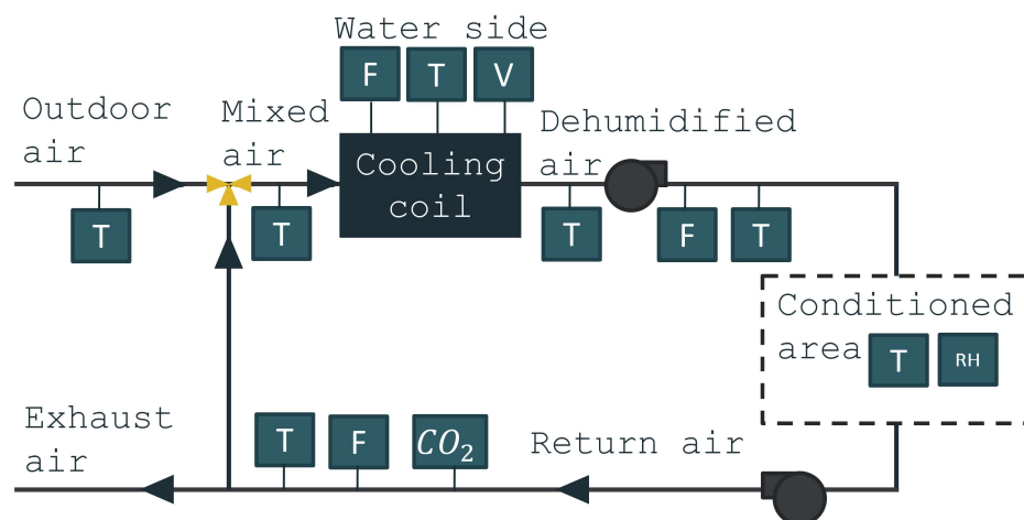
Fig. B.4.1.3 Air side system block diagram
